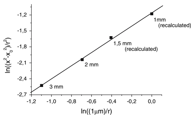
Fig. 7 Influence of radius of beads in the evolution of neck between soda-lime glass beads at 1.5 min. Where r is in \mu\text{m}
